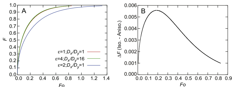
Fig. 3. (A) Comparison of fractional loss ( F ) as a function of Fourier number ( Fo ) for three hypothetical rectangular crystals of aspect ratio ( \varepsilon ) between 1 and 4. The \varepsilon = 4 rectangle has temperature-independent anisotropy, where diffusivity in longer crystallographic direction is 16\times faster than the shorter direction. Because the diffusivity in the longer direction is faster by a factor of \varepsilon^2 , diffusion proceeds at the same rate as from the \varepsilon = 1 rectangle with isotropic diffusivity. (B) Difference in F (isotropic-anisotropic) as a function of Fo . Geometric and diffusive anisotropy are indistinguishable to > 99\% , which is within the numerical uncertainty of the LB code at the resolution of these models ( 50 \times 50\varepsilon nodes).
