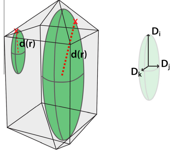
Fig. 9. Schematic illustration of the calculation of the normalized distance d(r) in a tetragonal prism with pyramidal terminations. The semi-axes of the ellipsoid centered at each point \mathbf{x} in the crystal are proportional to the tensor of diffusivity. The largest ellipsoid centered on \mathbf{x} that remains fully included into the crystal boundaries provides a measure of d(r) at this point. The volumetric average of d(r) yields the AND.
